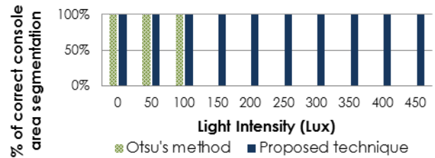
Figure 10 Percentage of correct console area segmentation comparing between the proposed technique and Otsu's method
