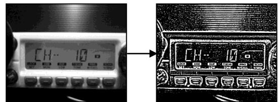
Figure 4 Adaptively thresholding the V-parameter gray-scale image to a binary image
