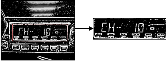
Figure 6 Selected console area using Blob detection
