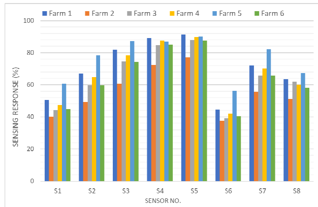
Fig. 4 Average percentage change in resistance of 8 semiconductor gas sensors used in electronic nose
